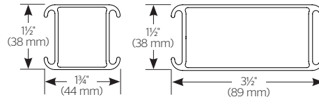
Standard Extrusion
